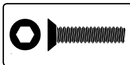
FLAT HEAD SCREWS - 10 PCS C-3002-30-06 M3x6 C-3002-30-08 M3x8 C-3002-30-10 M3x10 C-3002-30-12 M3x12 C-3002-30-14 M3x14 C-3002-40-10 M4x10 C-3002-40-12 M4x12 C-3002-40-14 M4x14 C-3002-40-16 M4x16 C-3002-40-18 M4x18
